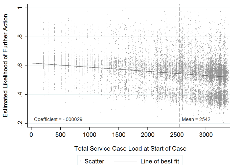
Figure 0.2 - Example Scatterplot
